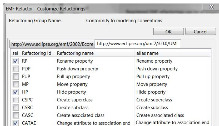
Figure 5: Existing refactorings can be configured into project-specific refactoring groups.
