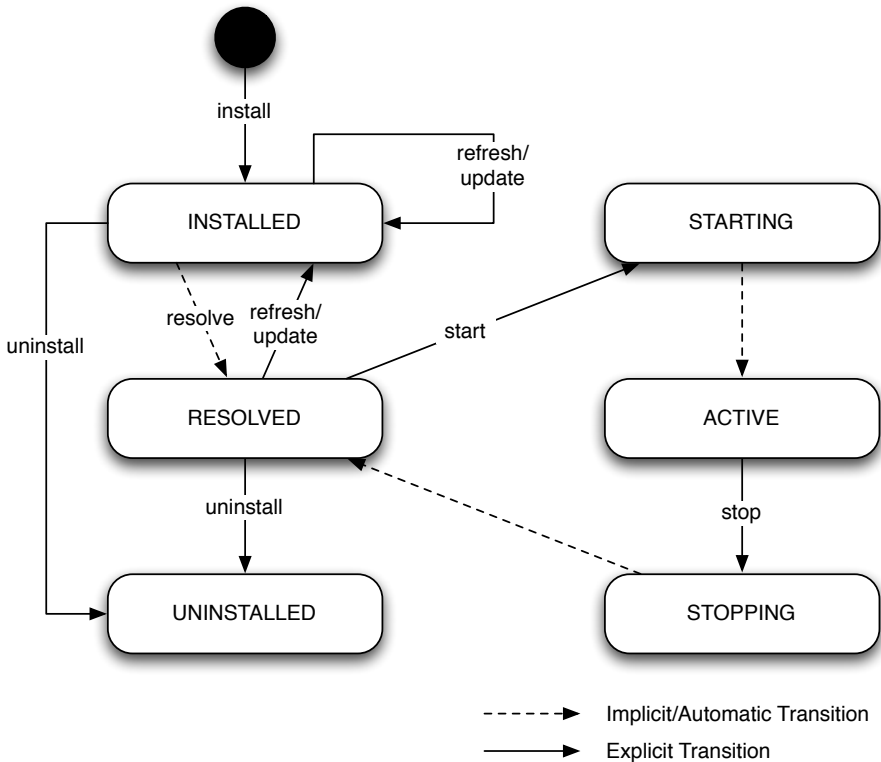
Figure 2.3.: Bundle Lifecycle
