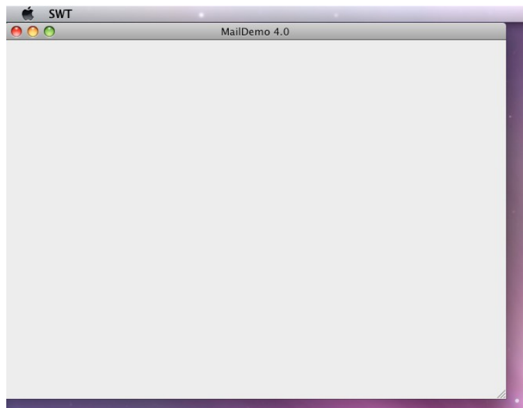
Figure 8: First Application
