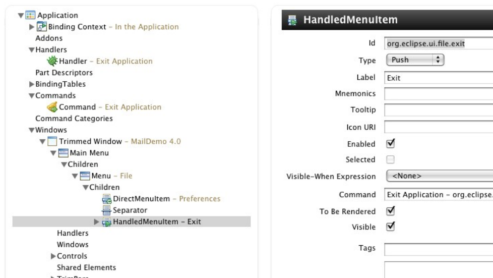
Figure 33: Model Structure
