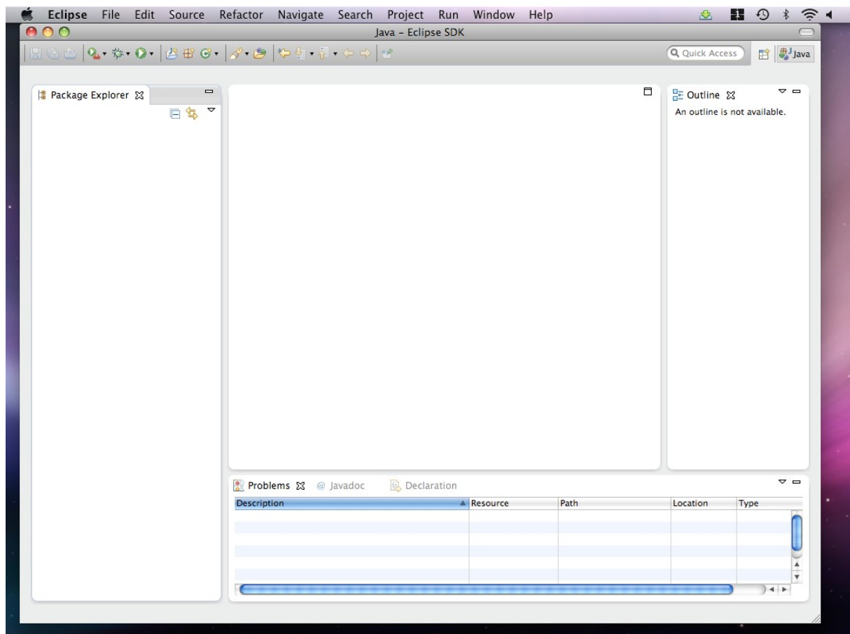
Figure 1: 4.1 SDK
