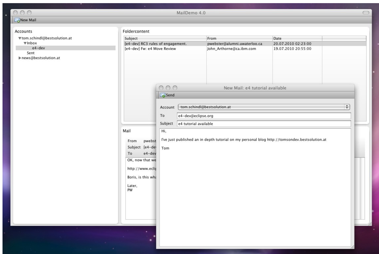
Figure 31: Final Application
