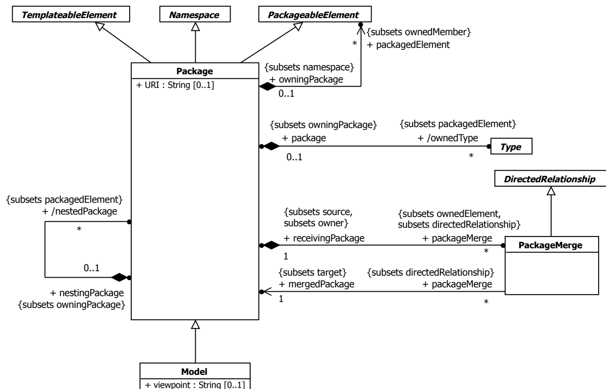
Figure 12.1 Packages
