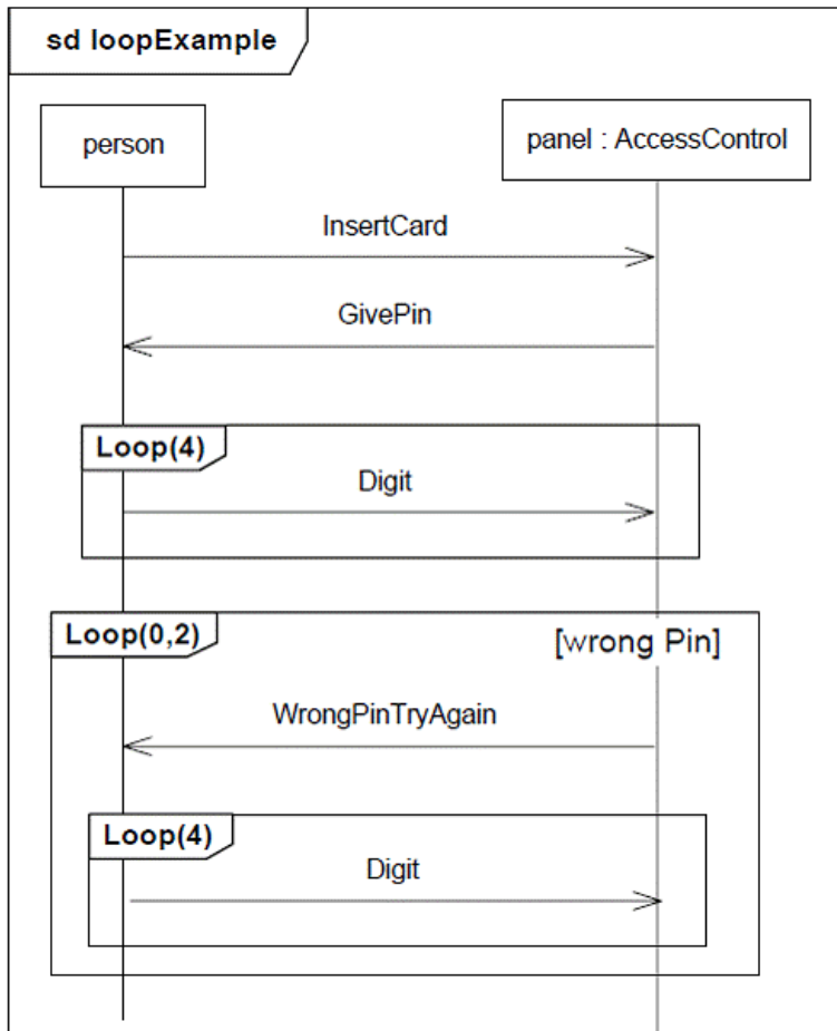
Figure 17.13 - Loop CombinedFragment
