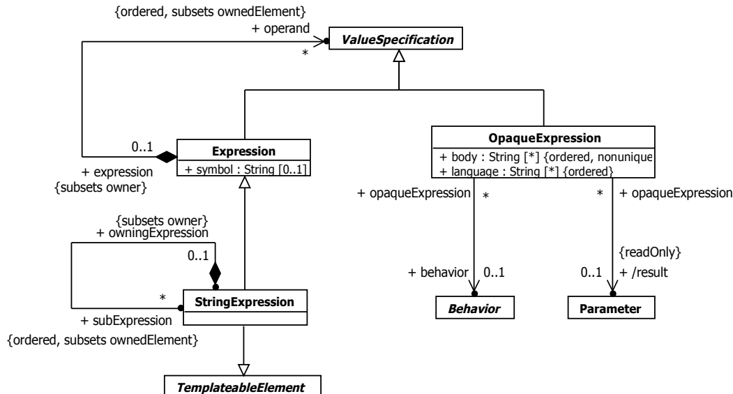
Figure 8.2 Expressions
