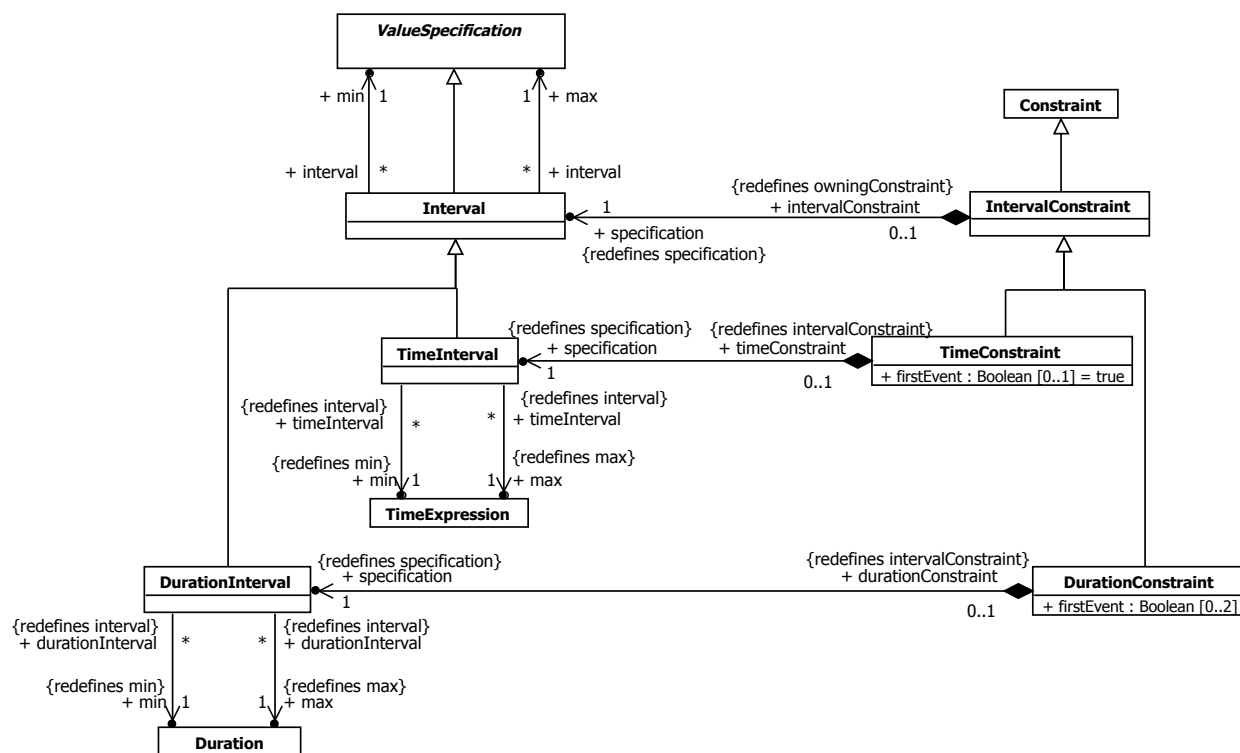
Figure 8.4 Intervals
