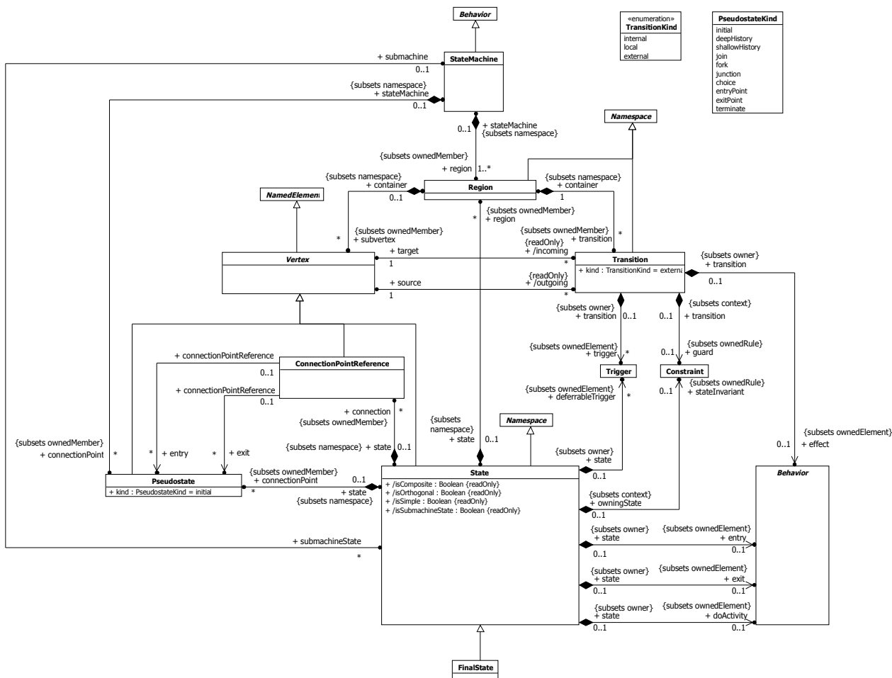
Figure 14.1 Behavior StateMachines
