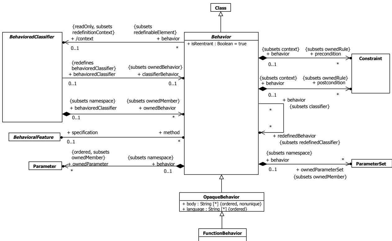
Figure 13.1 Behaviors
