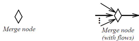
Figure 15.32 MergeNode notation
