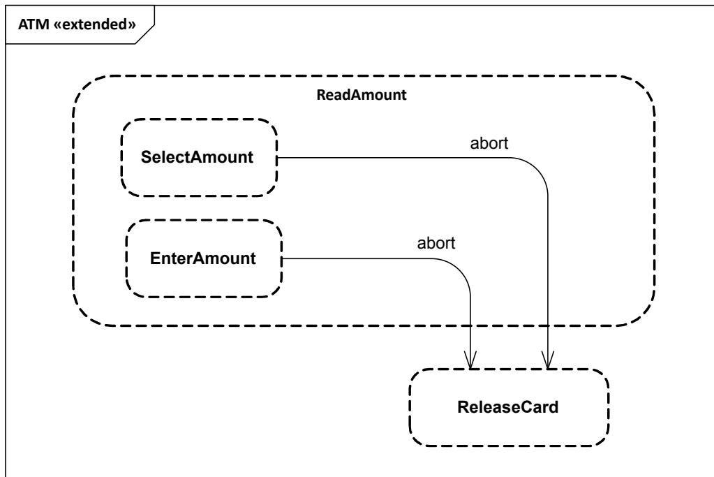
Figure 14.40 Adding Transitions
