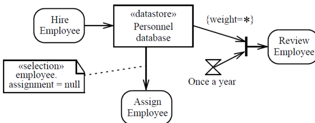
Figure 15.59 DataStoreNode example
