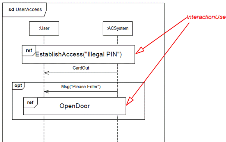
Figure 17.19 InteractionUse
