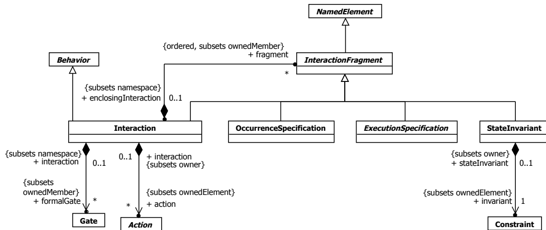
Figure 17.1 Interactions
