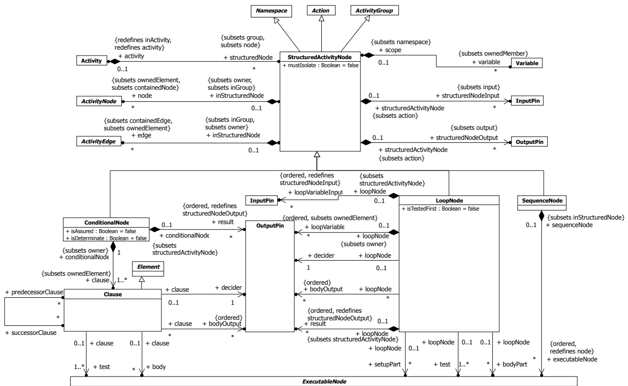
Figure 16.45 Structured Actions
