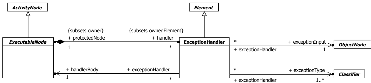
Figure 15.60 Executable Nodes
