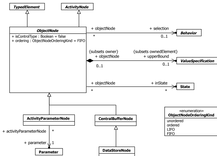
Figure 15.48 Object Nodes
