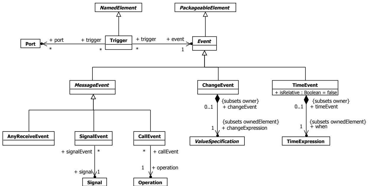
Figure 13.2 Events
