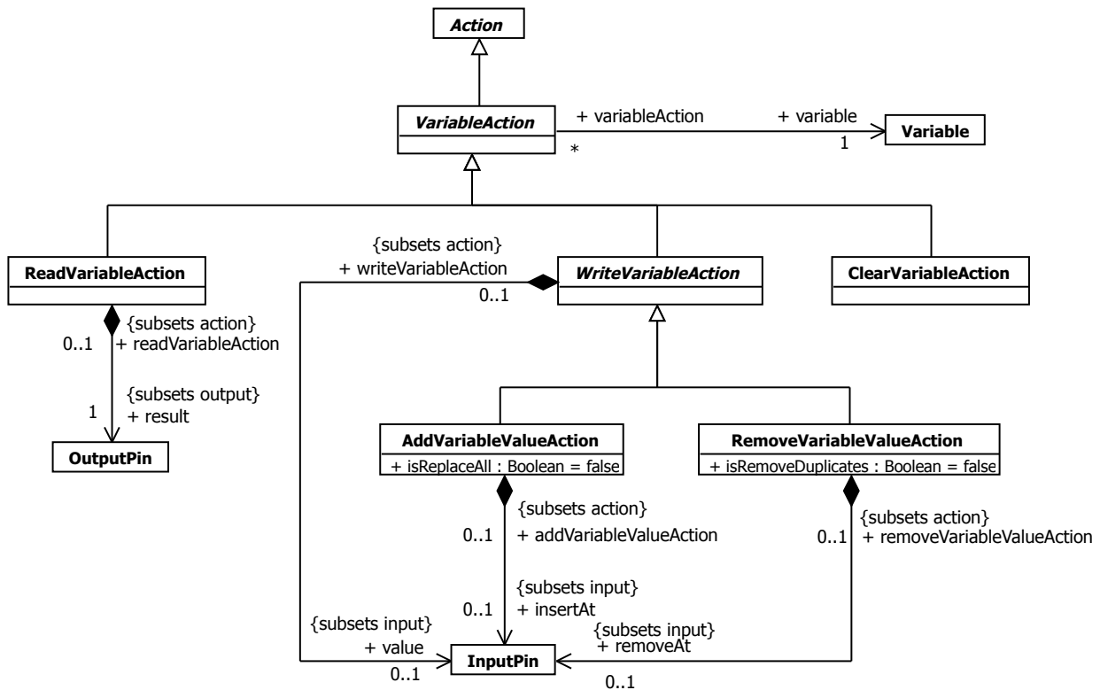
Figure 16.37 Variable Actions
