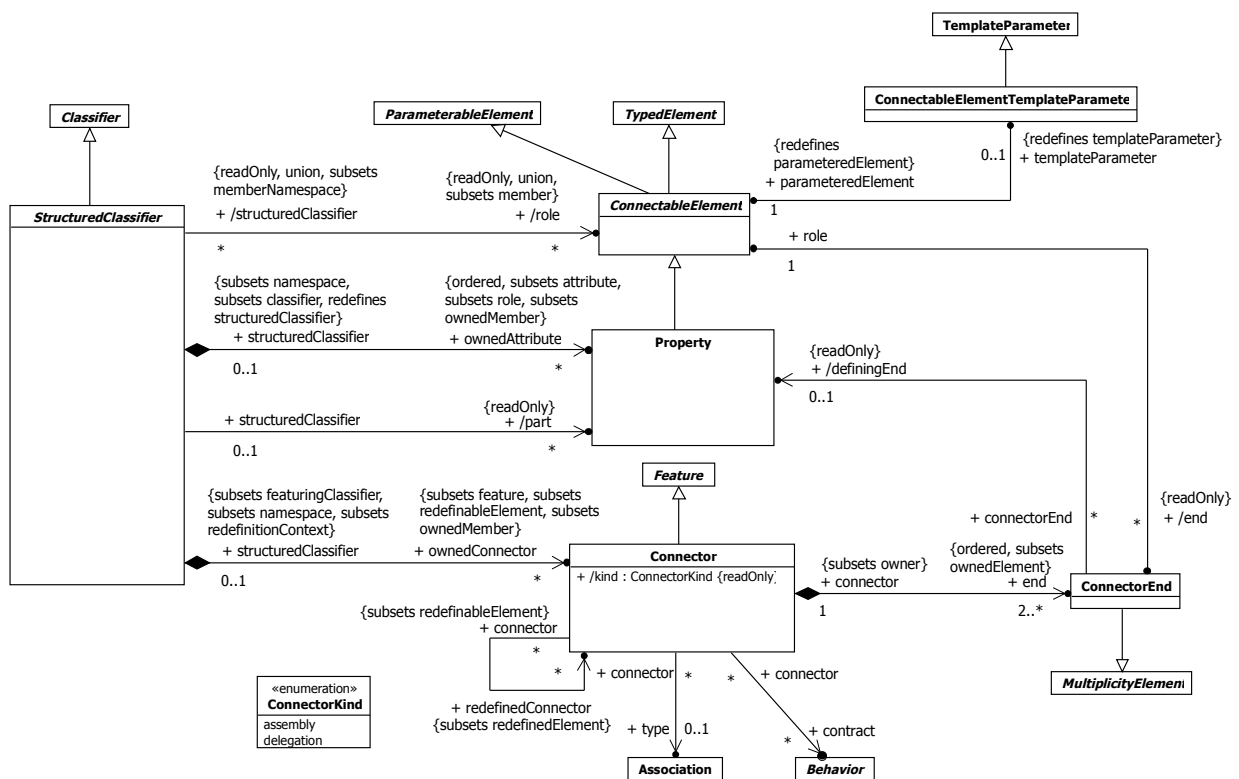
Figure 11.1 Structured Classifiers
