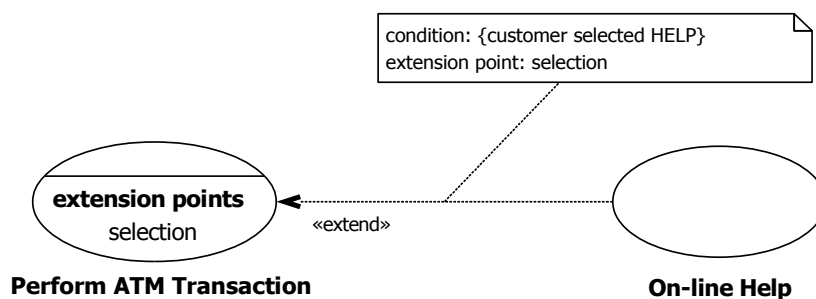
Figure 18.3 Example Extend
