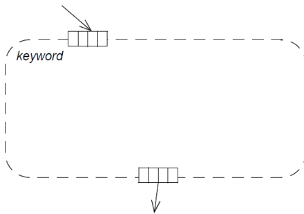
Figure 16.48 Expansion Region
