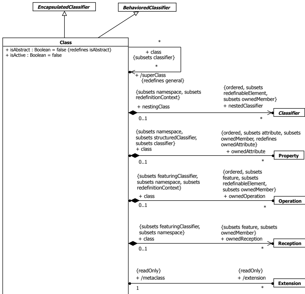
Figure 11.15 Classes
