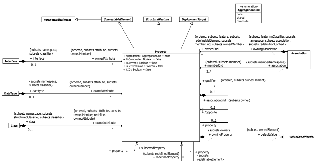
Figure 9.10 Properties
