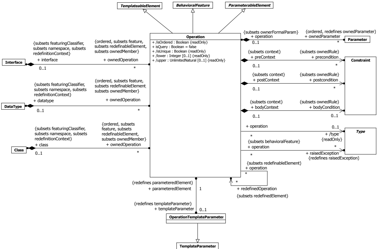
Figure 9.13 Operations
