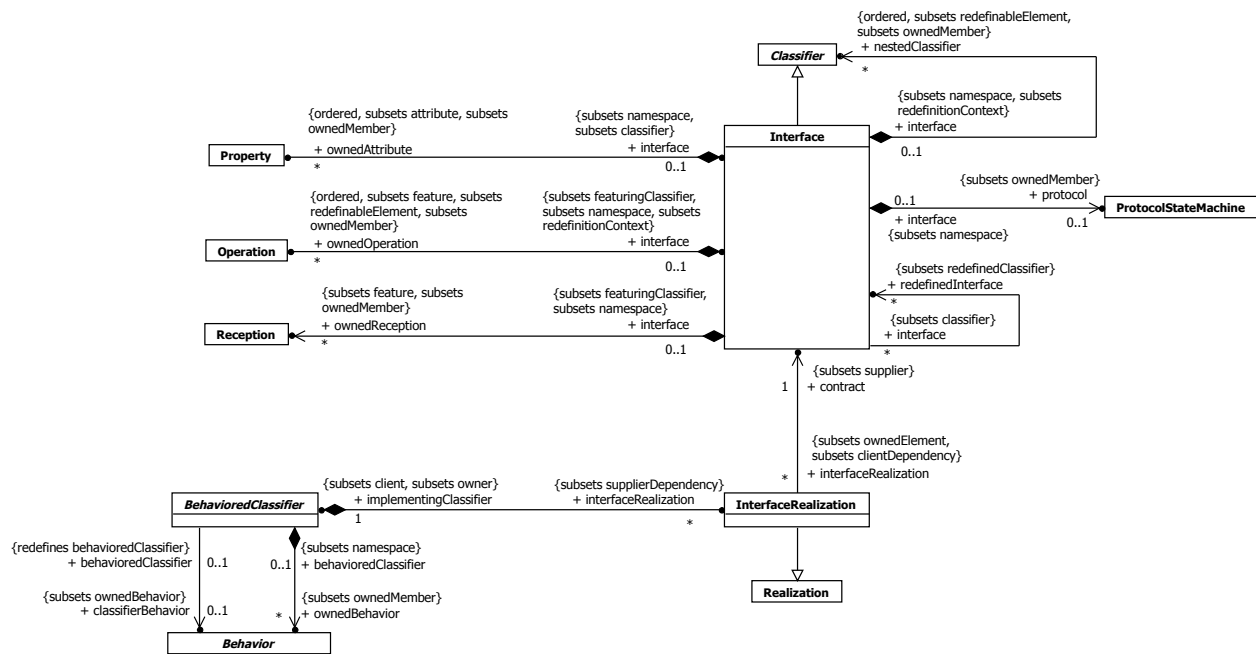
Figure 10.7 Interfaces
