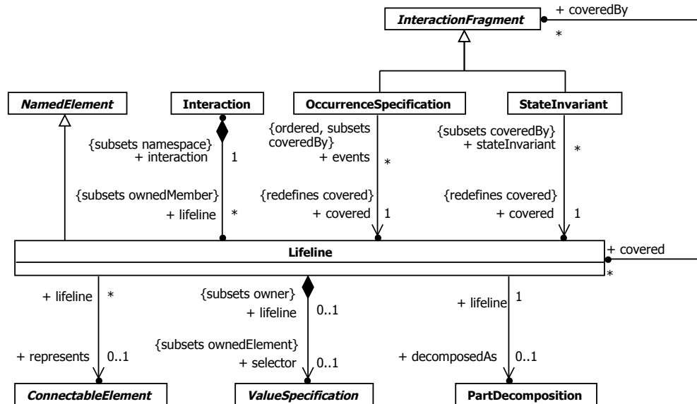
Figure 17.6 Lifelines
