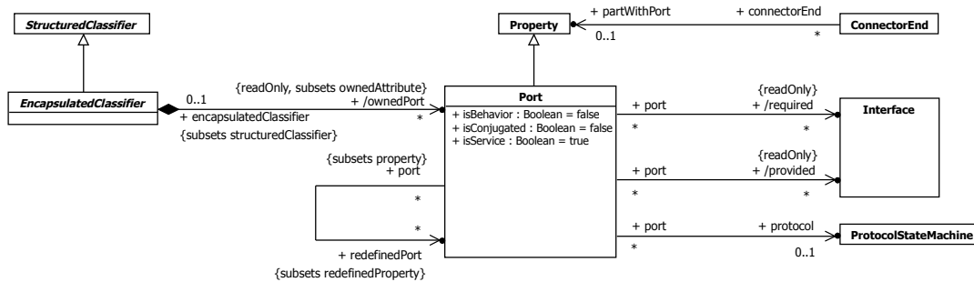
Figure 11.10 Encapsulated Classifiers
