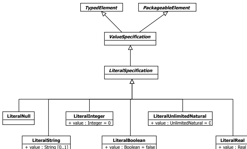
Figure 8.1 Literals
