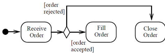
Figure 15.40 DecisionNode example
