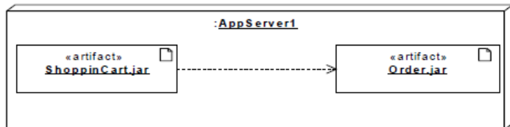
Figure 19.16 Deployed component Artifacts on a Node.
