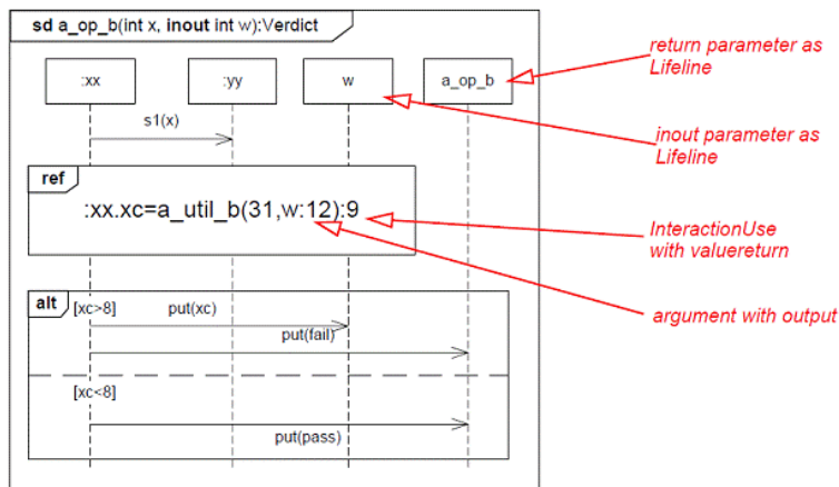
Figure 17.20 InteractionUse with value return
